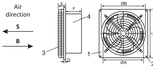
FIG. 1 - Installing the ventilator into a wall opening
